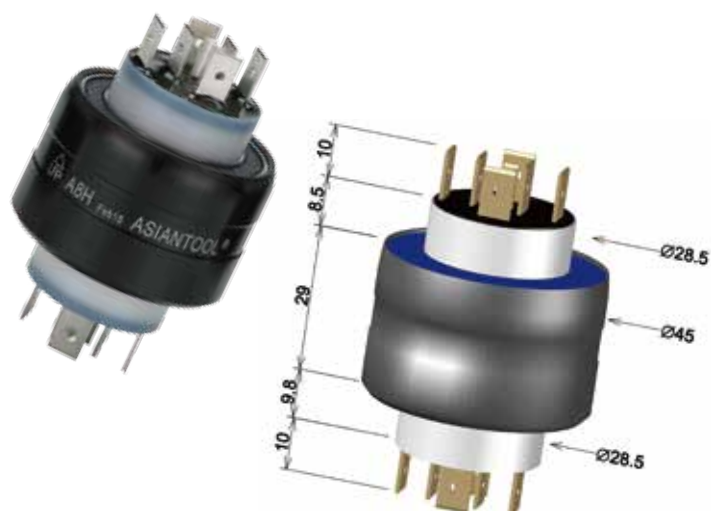
A8H 6poles/30A & 2poles/4A AC250V
