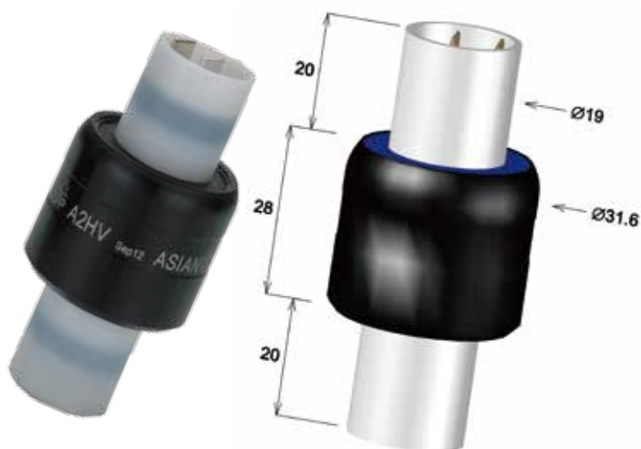
A2HV 2poles/30A/AC500V
