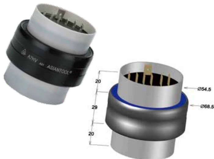
A7HV 7poles/30A/AC500V
